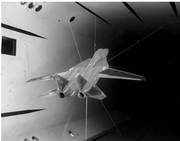
Fig. 3 F-14 model tested in TDT.
