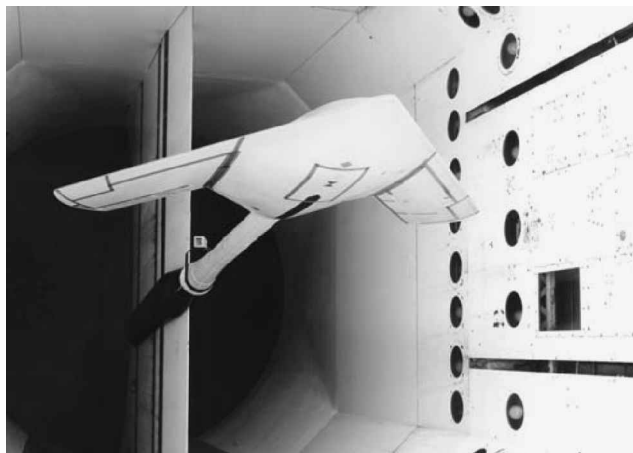
Fig. 17 Smart-wing UCAV model mounted on TDT sting.
