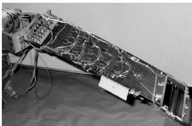
Fig. 12 Internal details of the PARTI model.
