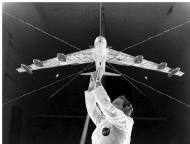
Fig. 10 B-52 model mounted on two-cable-mount system.
