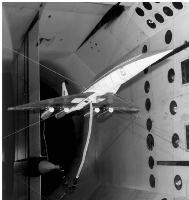
Fig. 14 SST model mounted on the two-cable-mount system.
