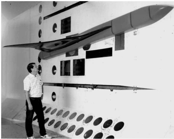
Fig. 19 HSR-RSM model mounted in the TDT.
