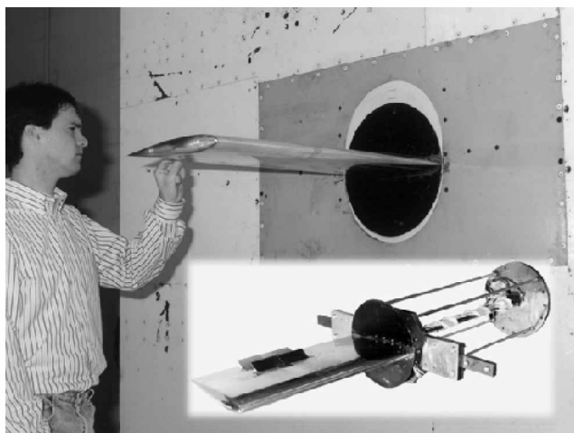
Fig. 13 BACT semispan model on the PAPA mount.
