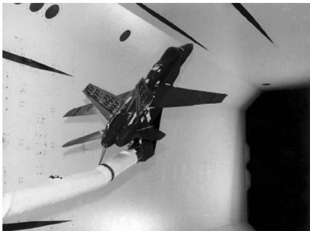
Fig. 15 BLA F-18 testbed on the TDT centerline sting.
