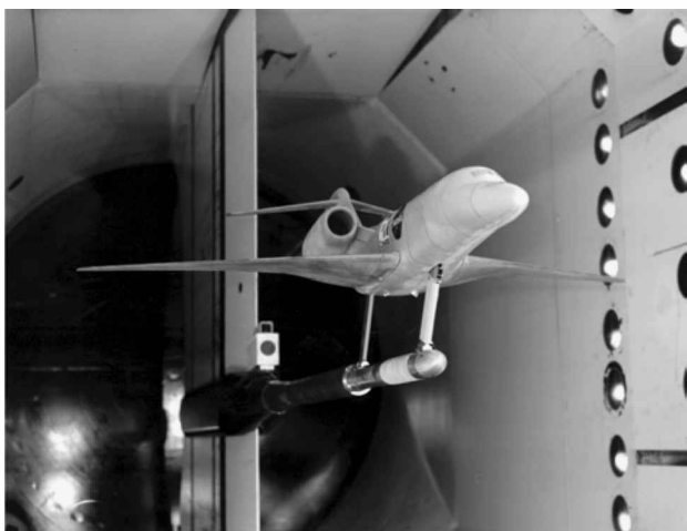
Fig. 7 Cessna Citation X business jet configuration in the TDT.
