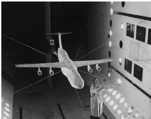
Fig. 9 C-5A model on two-cable-mount system.
