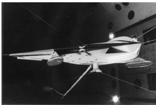
Fig. 6 Cable-mounted A-12 configuration.
