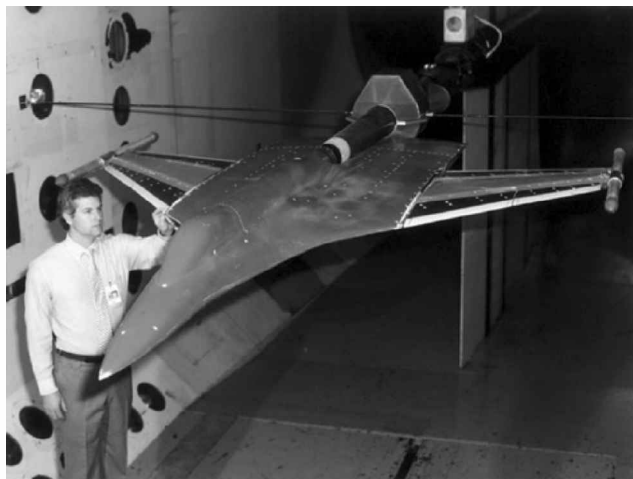
Fig. 11 AFW model mounted on free-to-roll rig.
