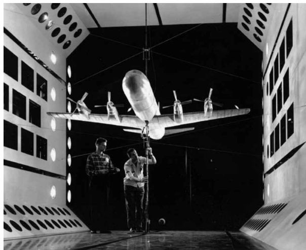
Fig. 1 Lockheed Electra model mounted in the TDT.
