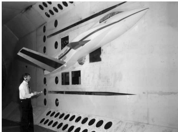
Fig. 5 Grumman X-29 model mounted to TDT sidewall support system.
