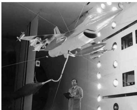
Fig. 4 F-16 fighter configuration in TDT.
